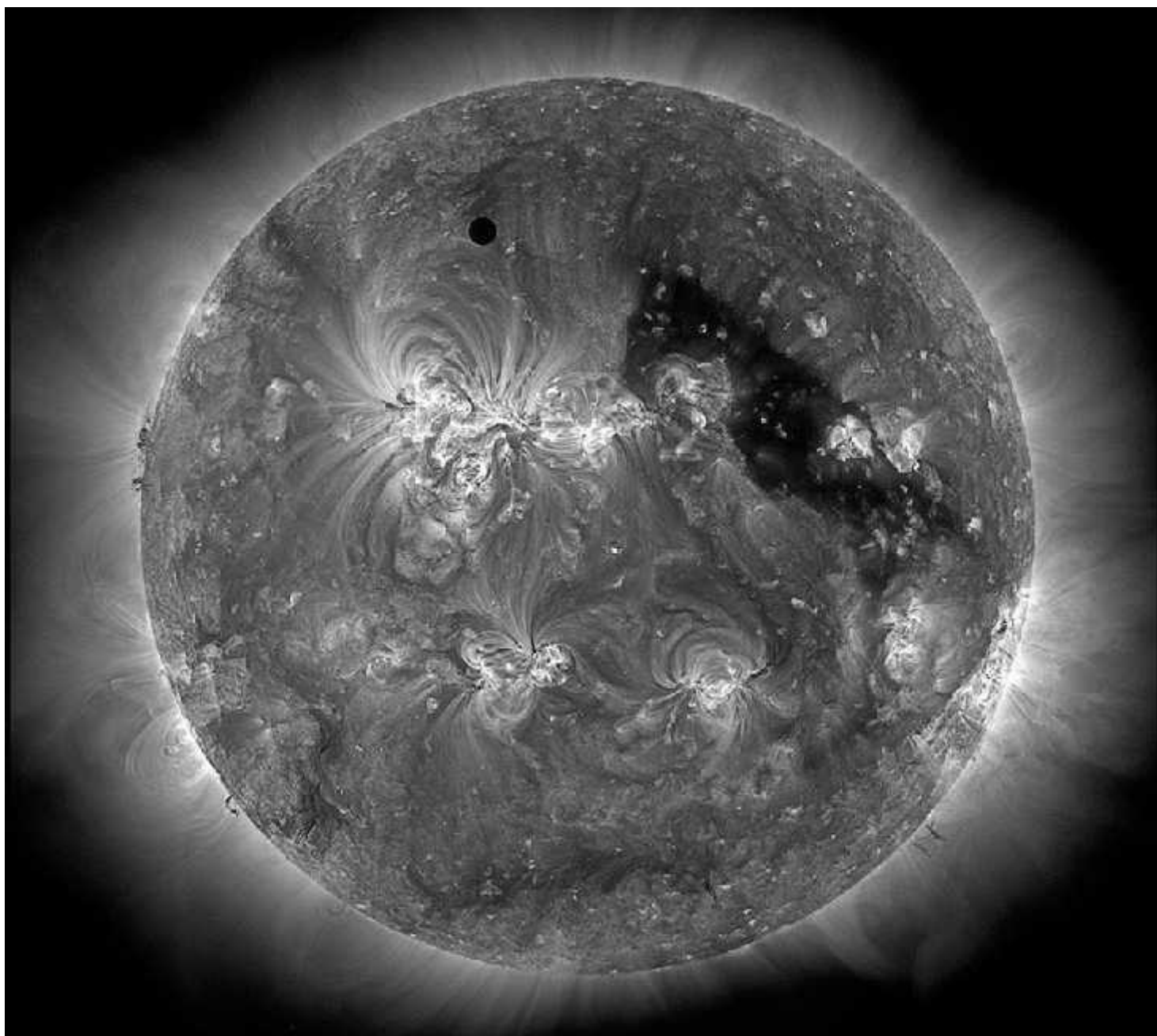
Venus and the Triply Ultraviolet Sun Image Credit: NASA/SDO & the AIA, EVE, and HMI teams; Digital Composition: Peter L. Dove
